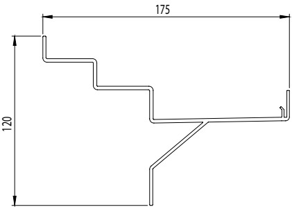
TERMINAL TUBE
