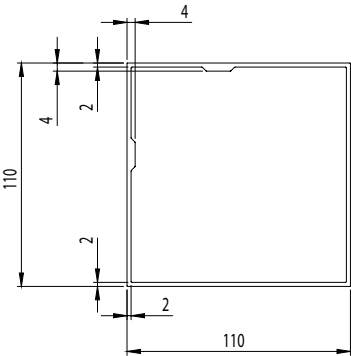
FRONT AND REAR COVER PROTECTION
